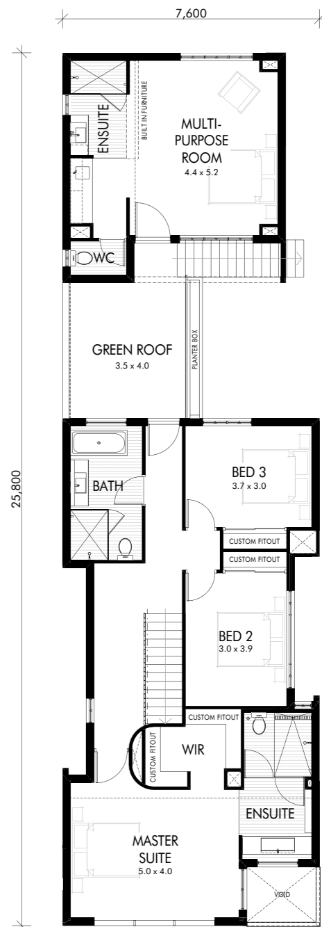
UPPER FLOOR
