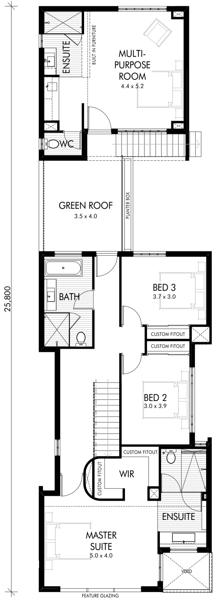
UPPER FLOOR PLAN
